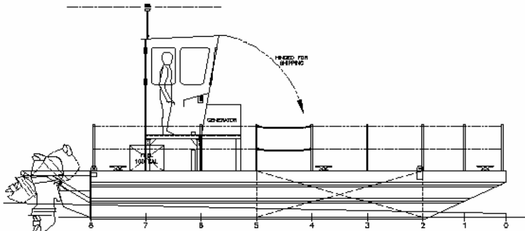
OUTBOARD PROFILE
